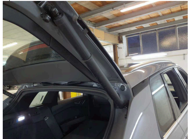
Damage #2: Boot lid / rear door: Gas pressure damper - Worn - Replace
