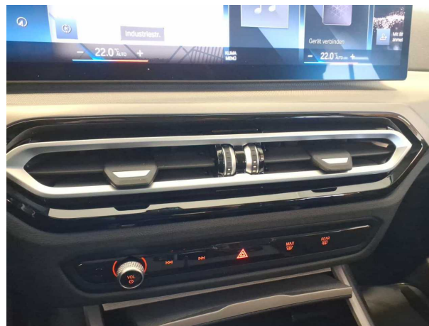
Illustration 8: Habitable
