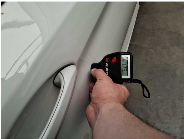
Repainting 3: Door - front right side
